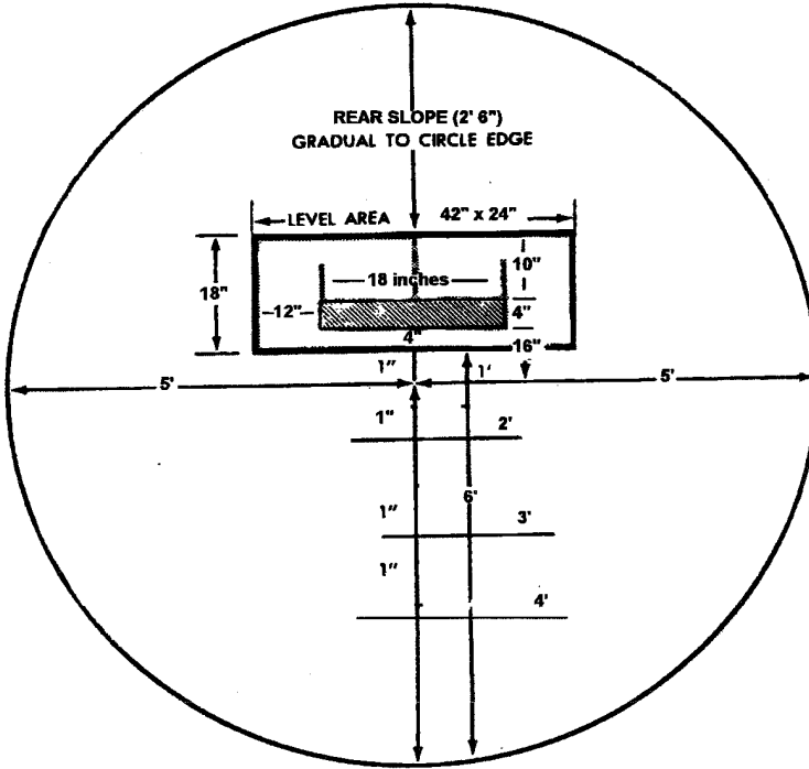
Little League Baseball Pitching Mound Layout
